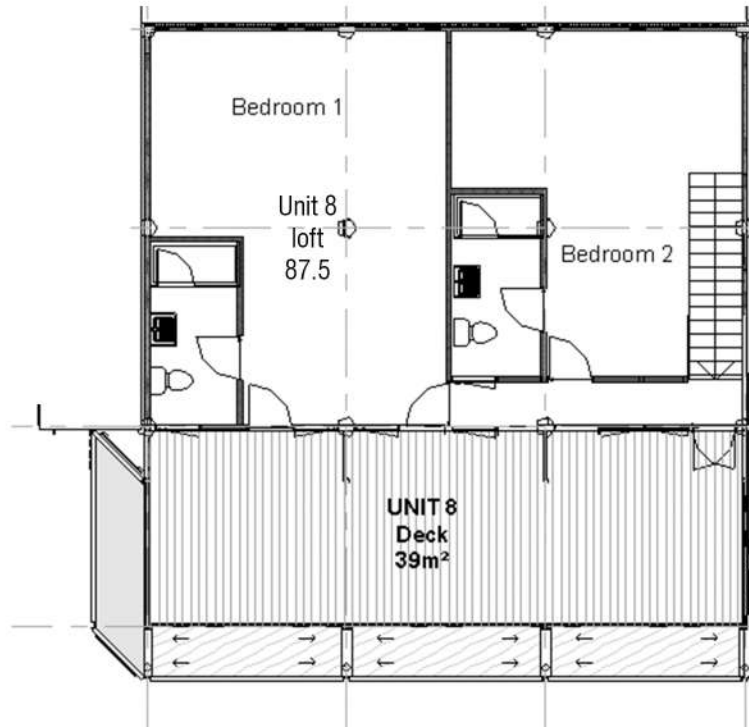
LOFT FLOOR PLAN NTS.
