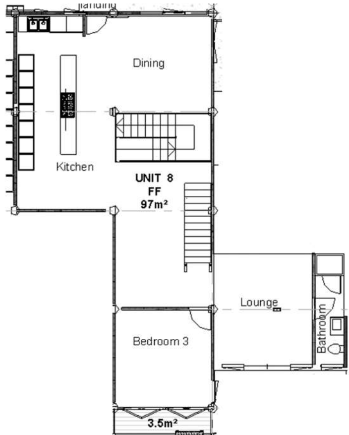
FIRST FLOOR PLAN NTS.
